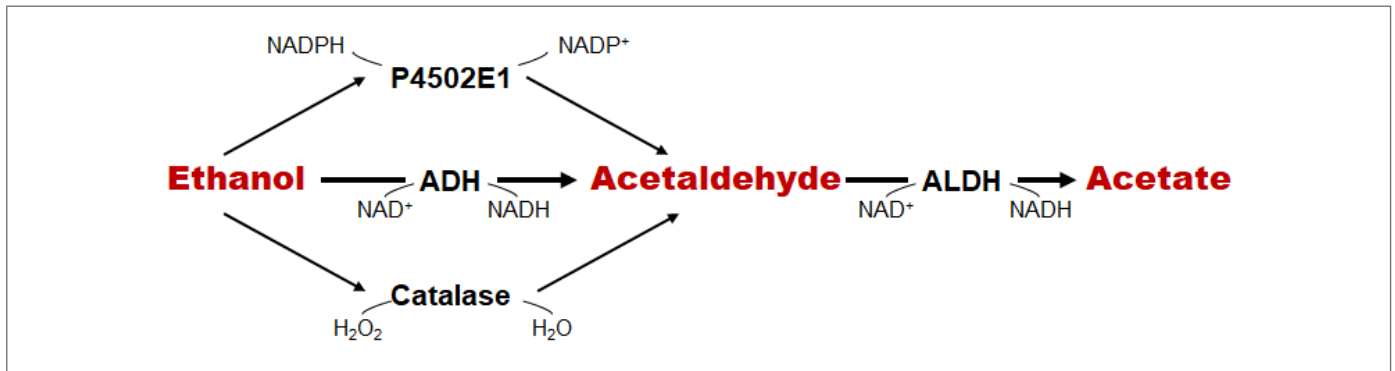
Figure 1. Alcohol metabolism
